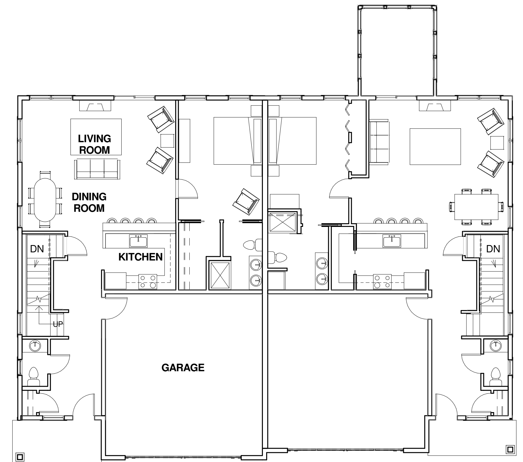
5 | B - FIRST FLOOR PLAN 1/8" = 1'-0"
