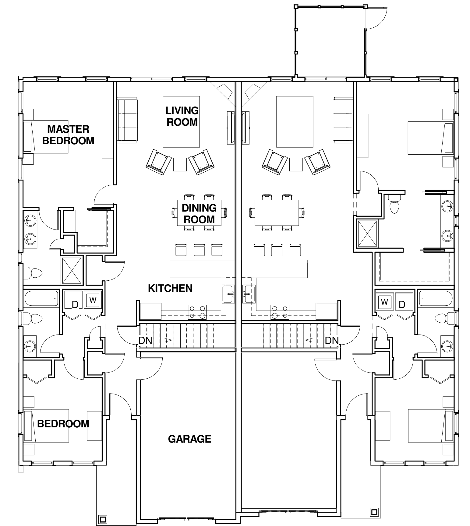
5 | A - FIRST FLOOR PLAN 1/8" = 1'-0"
