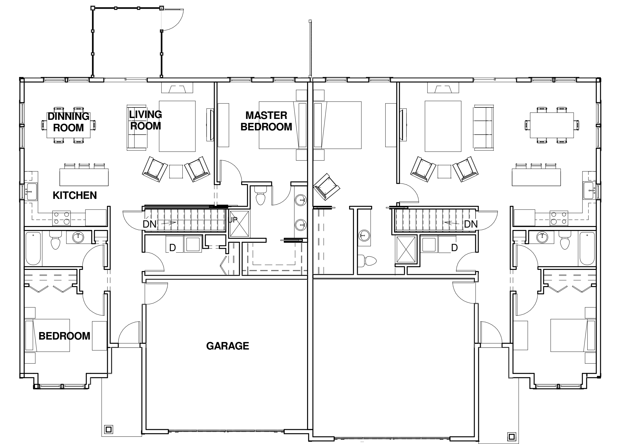
5 | C - FIRST FLOOR PLAN 1/8" = 1'-0"
